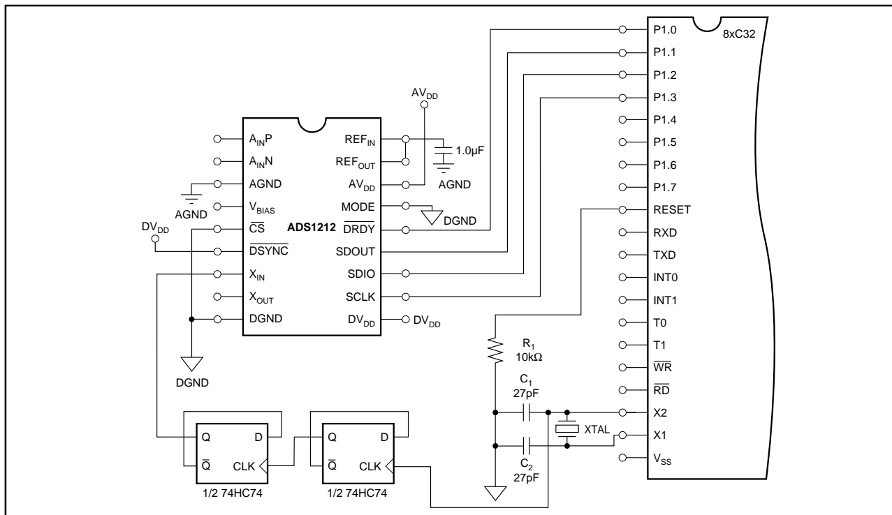
FIGURE 30. Four-Wire Interface with a 8xC32 Microprocessor.
