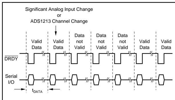
FIGURE 4. ADS1212/13 Analog Input Voltage Step or ADS1213 Channel Change to Fully Settled Output Data.
