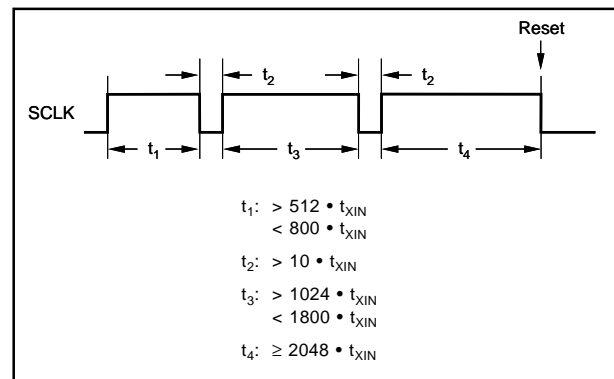
FIGURE 27. Resetting the ADS1212/13 (Slave mode only).
